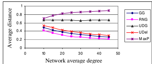
Fig. 2. Average transmission distance
