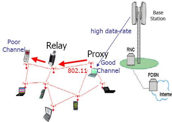
Fig. 1. Integrated Cellular and Ad-Hoc Networks
