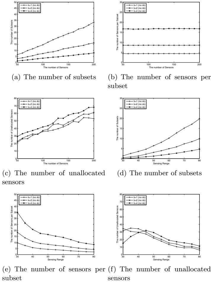
Fig. 3. Effect of total number of sensors and the sensing range on the network lifetime. Density Control is NOT applied.
