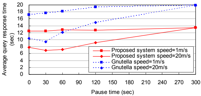
Fig. 2. Average query response time
