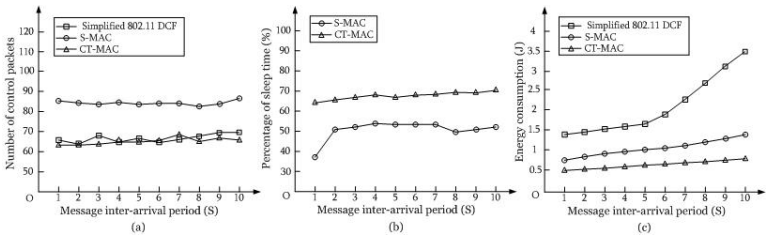
Fig. 7. The measured number of control packets(a), the percentage of sleep time(b), and the energy consumption(c)
