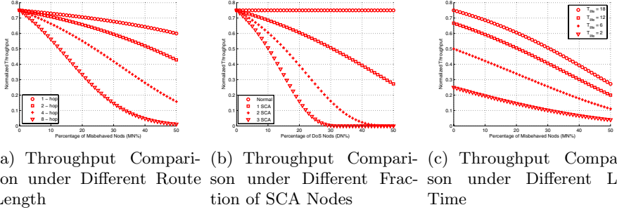
Fig. 4. Impacts of SCA combined with DoS Attacks
