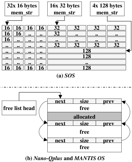
Fig. 1. Memory management data structures on SOS , Nano-Qplus , and MANTIS OS
