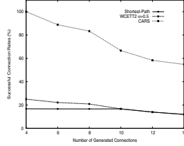
Fig. 7. Successful connection rates w/ 80 mesh routers (3 work as gateways), CBR, 2 NICs & 3 exclusive channels, outdoors
