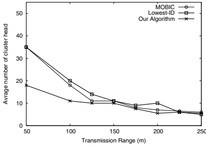
Fig. 4. Comaprisn between different clustering algorithms
