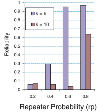
Fig. 10. Performance of pbcst ( p = 0.8 ) with repeaters for 441 motes deployed with inter-mote density s = 6' and 10'
