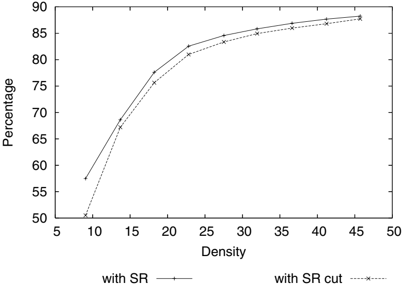
Fig. 2. Improvement by using Source Routing
