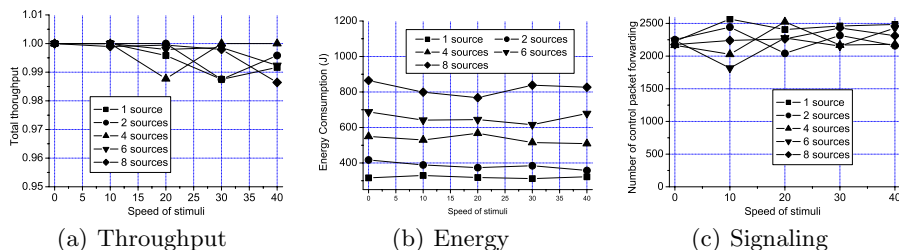
Fig. 6. Impact of the number and the speed of the stimuli
