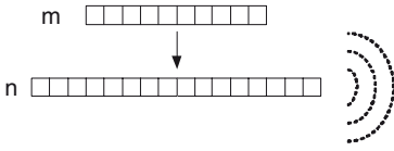
Fig. 1. FBcast at source: m original packets are encoded into n packets and injected in the network
