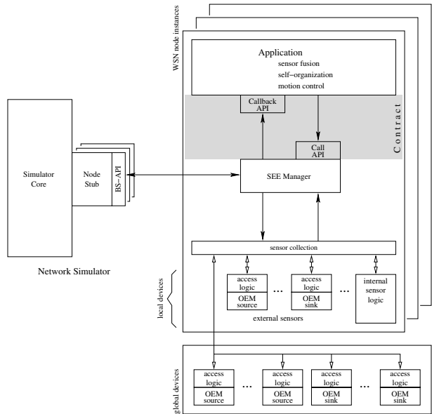
Fig. 3. SEE architecture
