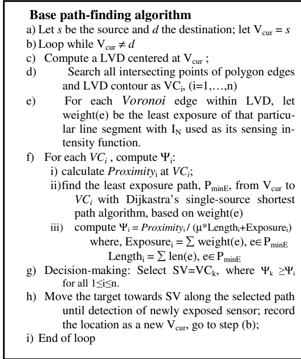
Fig. 3. Pseudo-code of the base path-finding algorithm
