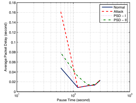
(b) Average Packet Delay
