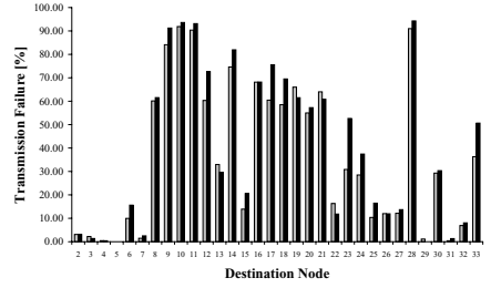
Fig. 10. Transmission failures in percent with (gray) and without (black) XTC
