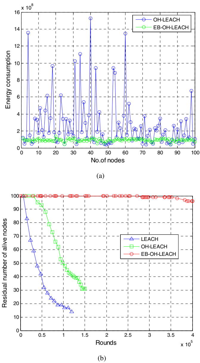
Fig. 3. Energy consumption (a) and Network lifetime (b) by OH-LEACH and EB-OH-LEACH
