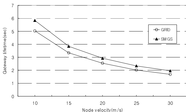
Fig. 9. Gateway lifetime varied by velocity
