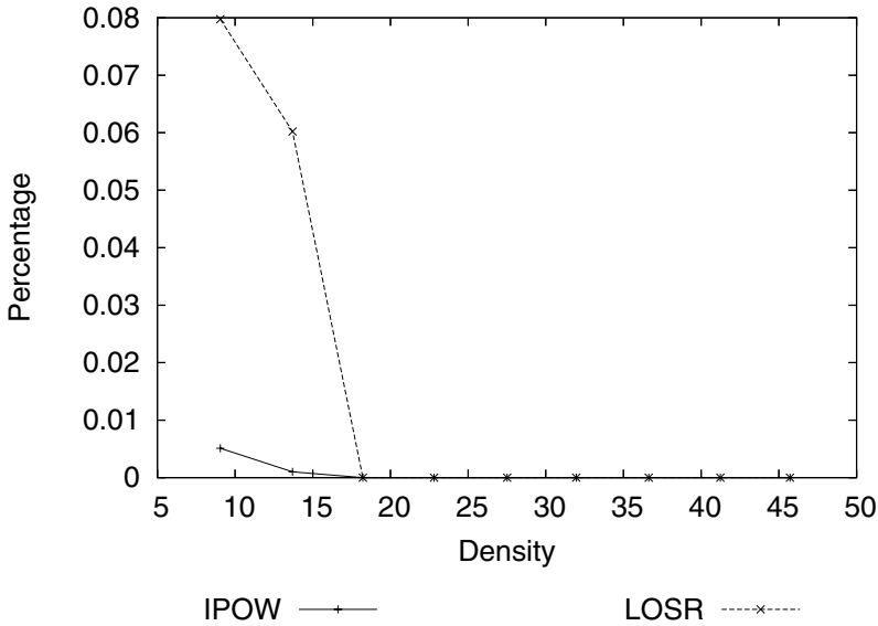
Fig. 5. Percentage of messages sent in perimeter mode
