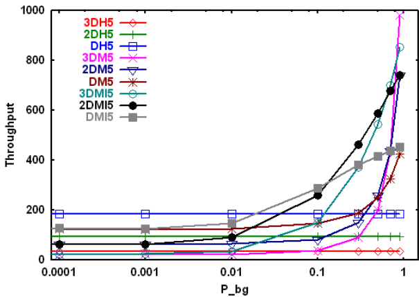
(c) five-slot packet type
