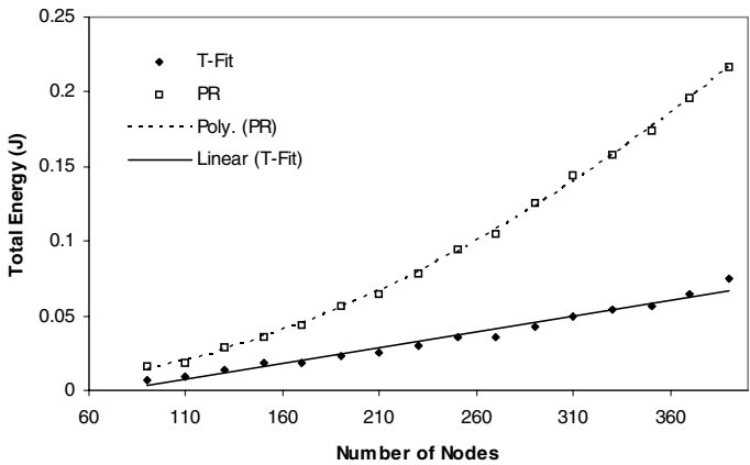
Fig. 8. Total energy dissipation against number of nodes for a 35-m circular event area and nodes with 15-m radio range
