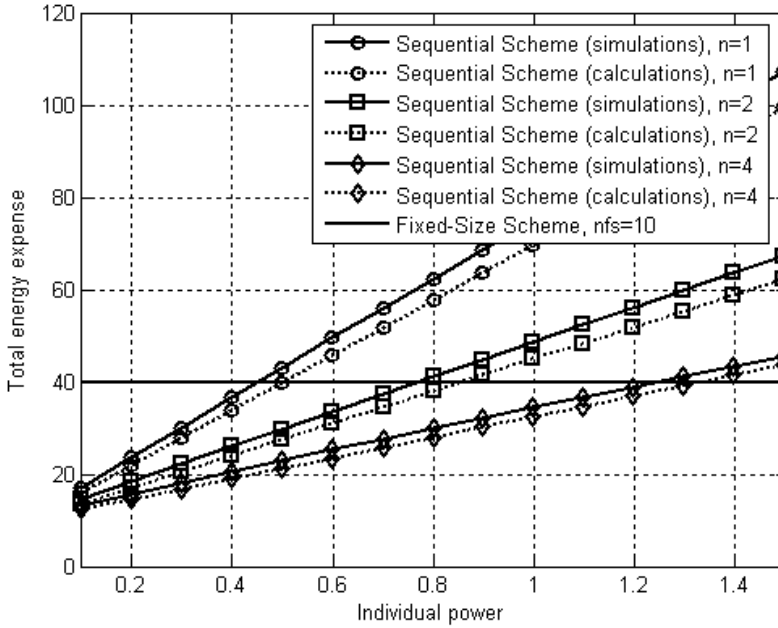
Fig. 2. Average energy expenses for data transmission
