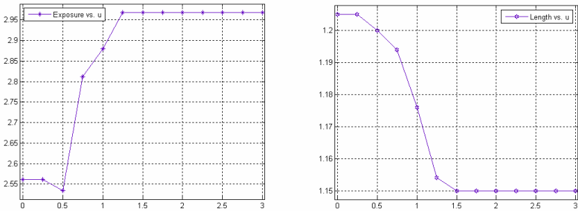
Fig. 7. FDP Performance vs. \mu ( N=110, r_D=320 )
