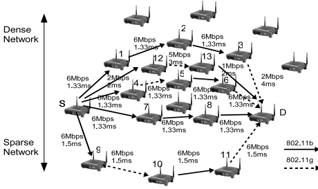
Fig. 1. 5 candidate routes from source S to destination D
