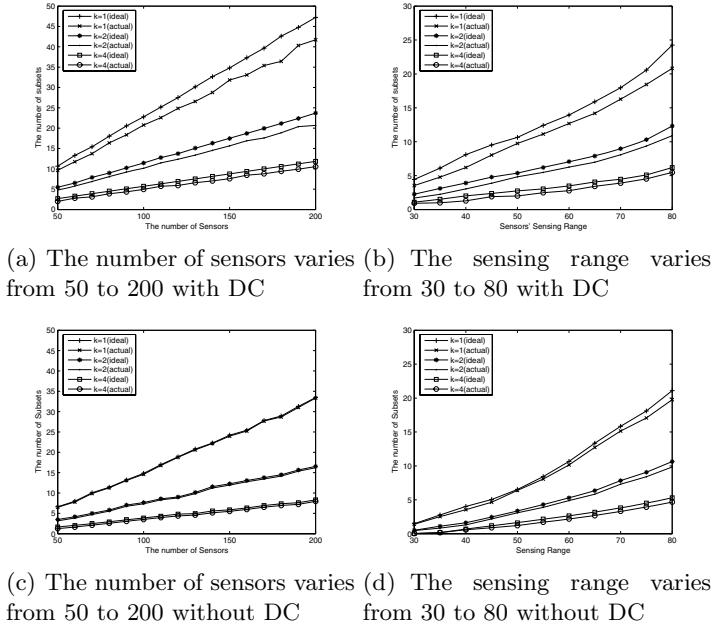
Fig. 2. Compare GS's results with the ideal results
