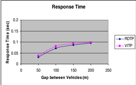
Fig. 7. Response time vs. vehicle gap
