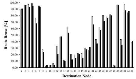
Fig. 12. Percentage of route reuse for communication with (gray) and without (black) XTC
