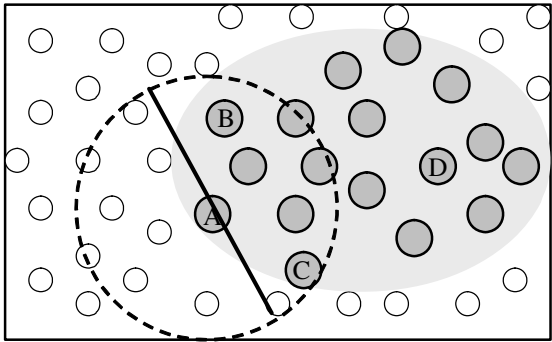
Fig. 2. A convex event-affected region is shown as a shaded area with affected nodes. Dashed circle centred at node A represents its radio range. A tangent segment is drawn on node A parallel to its farthest affected neighbours of B and C. From this tangent-fit test, node A is an edge node.
