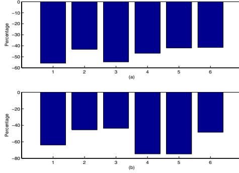
Fig. 3. Gain/Loss of distributed algorithms over their centralized counterparts: (a). Total average rate; (b). Effective rate; 1. MPF ( r_{II} ), 2. MQR ( r_{II} ), 3. MPF ( r_{III} ), 4. MQR ( r_{III} ), 5. MPF ( r_{IV} ), 6. MQR ( r_{IV} )
