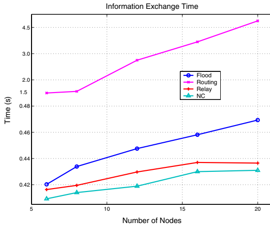
Fig. 8. Time Consumption after Information Exchange (Random Topology)
