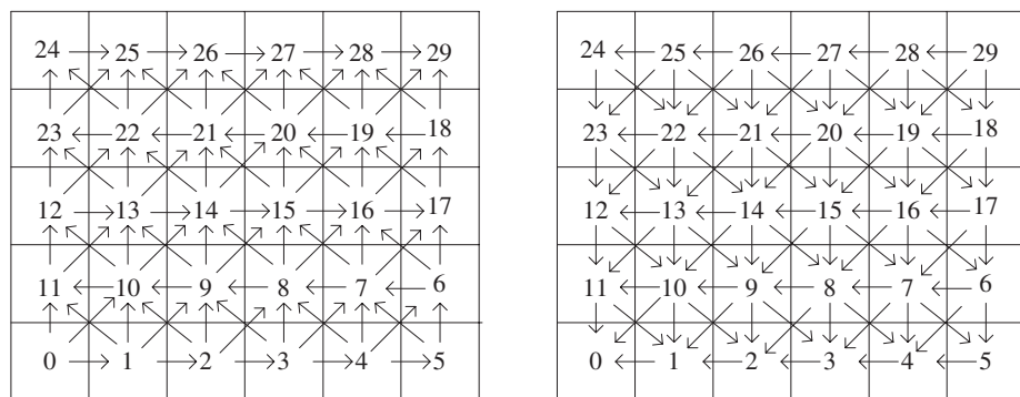
(a) High-channel subnetwork
