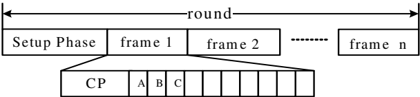
Fig. 2. Frame structure of BMA protocol
