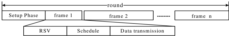
Fig. 3. Frame structure of ED-TDMA
