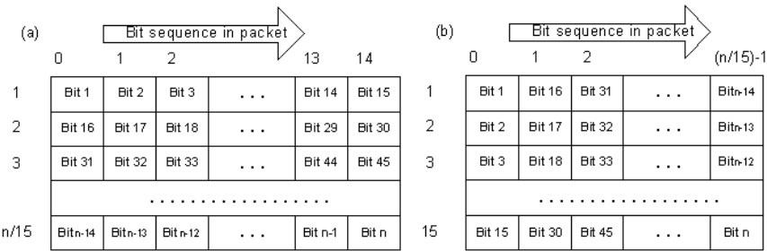
Fig. 4. The proposed link layer bit arrangement for Bluetooth EDR: (a) FEC coding (b) Interleaved FEC coding
