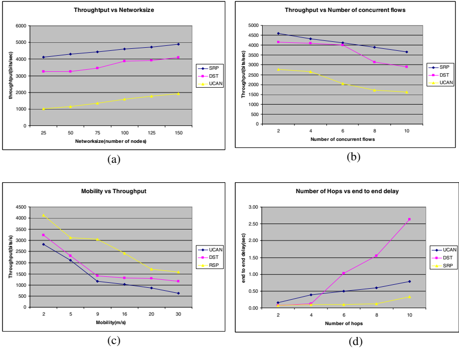
Fig. 8. Network throughputs and delay performance
