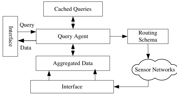
Fig. 1. Framework for History-based query processing
