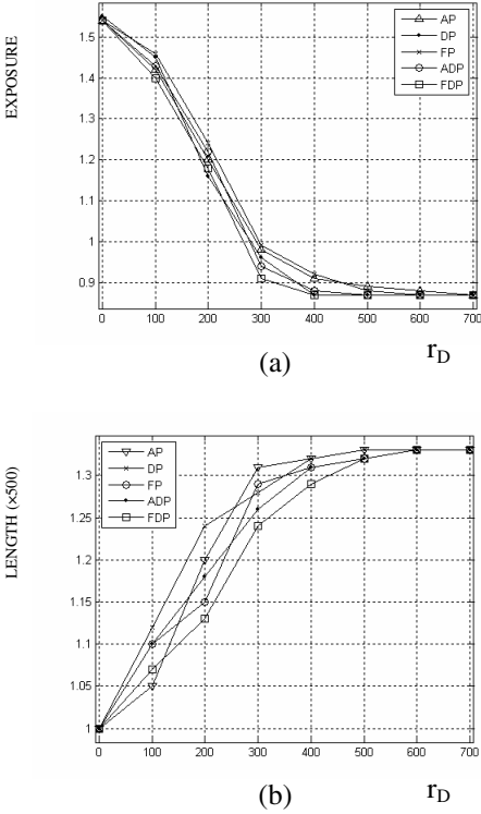
Fig. 6. Performance vs. Detection Radius ( N=50, \mu=0.5 )
