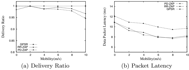
Fig. 8. Mobility Impact on Routing Performance
