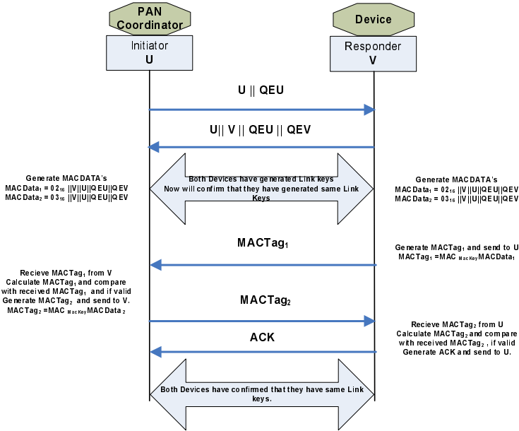
Fig. 4. Confirmation of Link Keys
