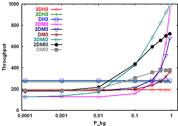
(b) three-slot packet type
