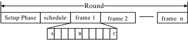
Fig. 1. Frame structure of traditional TDMA protocol
