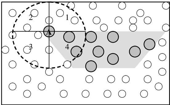
Fig. 3. A convex trapezoidal region that may have been bounded by a non-natural artifact. Node A is a valid edge node with all its affected neighbours populated only in the fourth quadrant.
